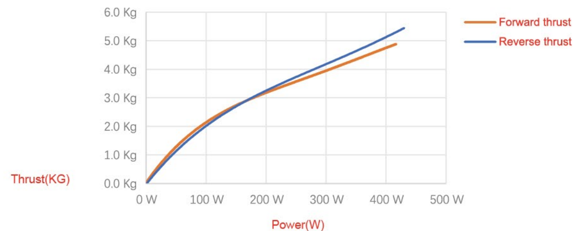
Thrust vs Input power table 2
